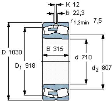
Tapered bore, taper 1: 30
